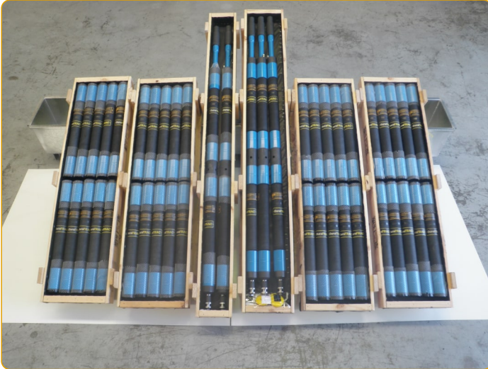
A shipment of customised 70mm Hydraulic Fracture Straddles with special 400mm long elements for a major South American mine in 2013. Now a standard product.
